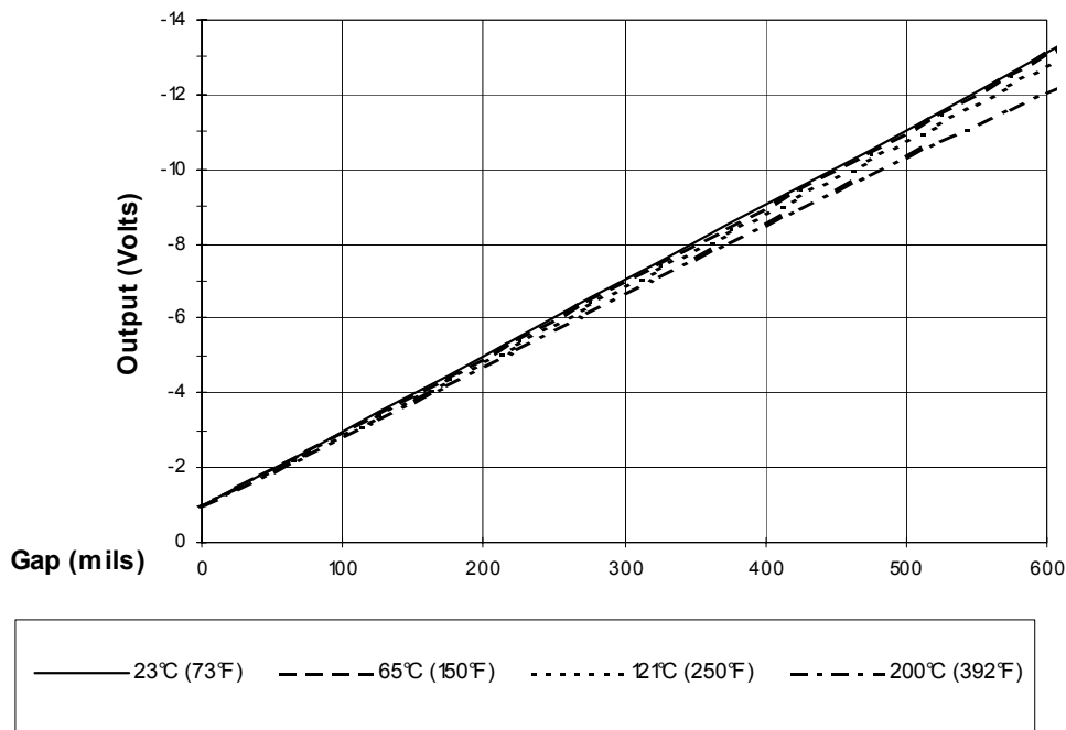
Figure 4 Typical 3300 XL 25 mm Probe + 1m Cable @ High Temperature (Proximator® Sensor + 4m of Extension Cable @ 25 °C)
