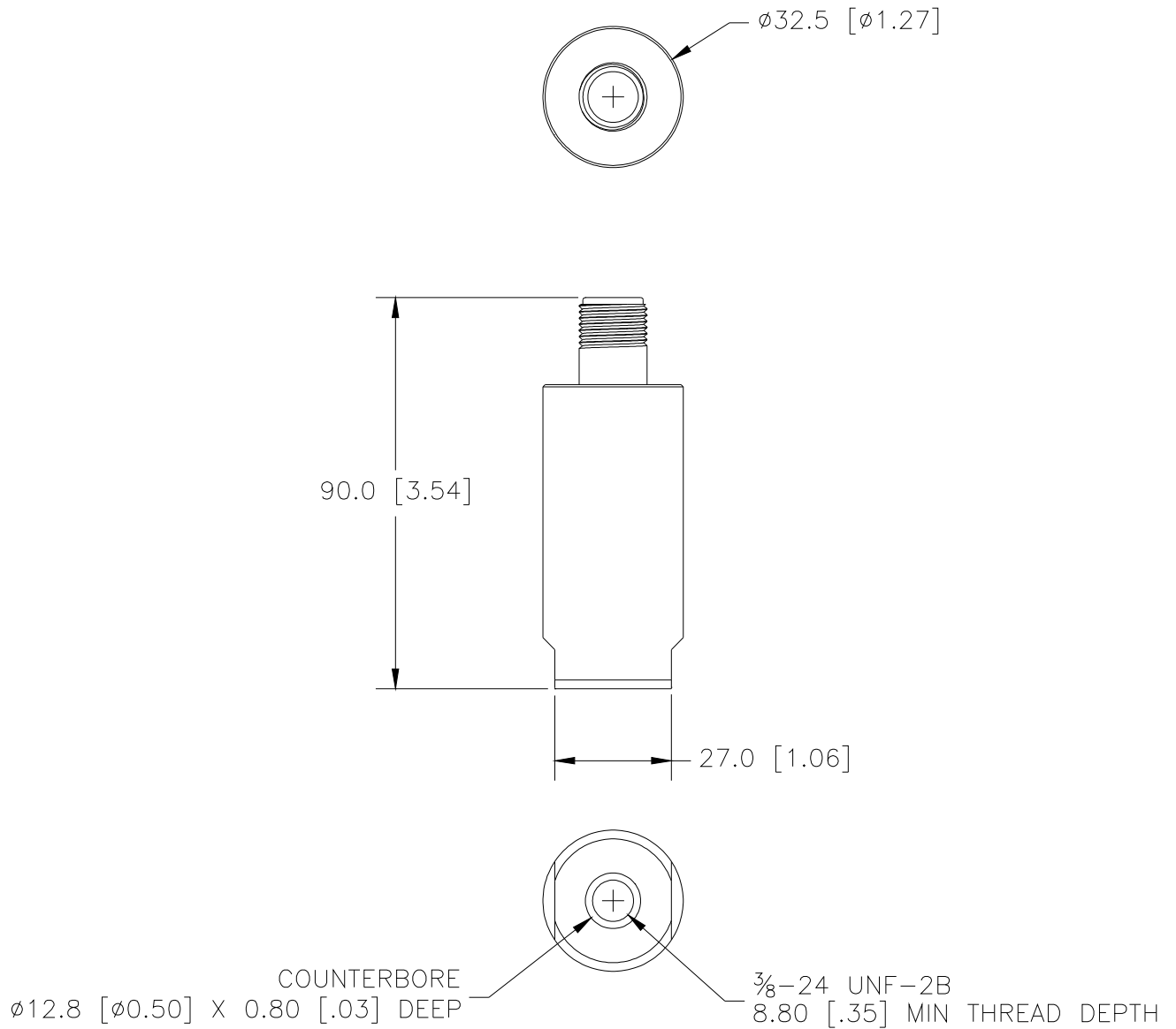
Figure 2: 330505 System Dimensional Drawing Dimensions are in millimeters (inches)
