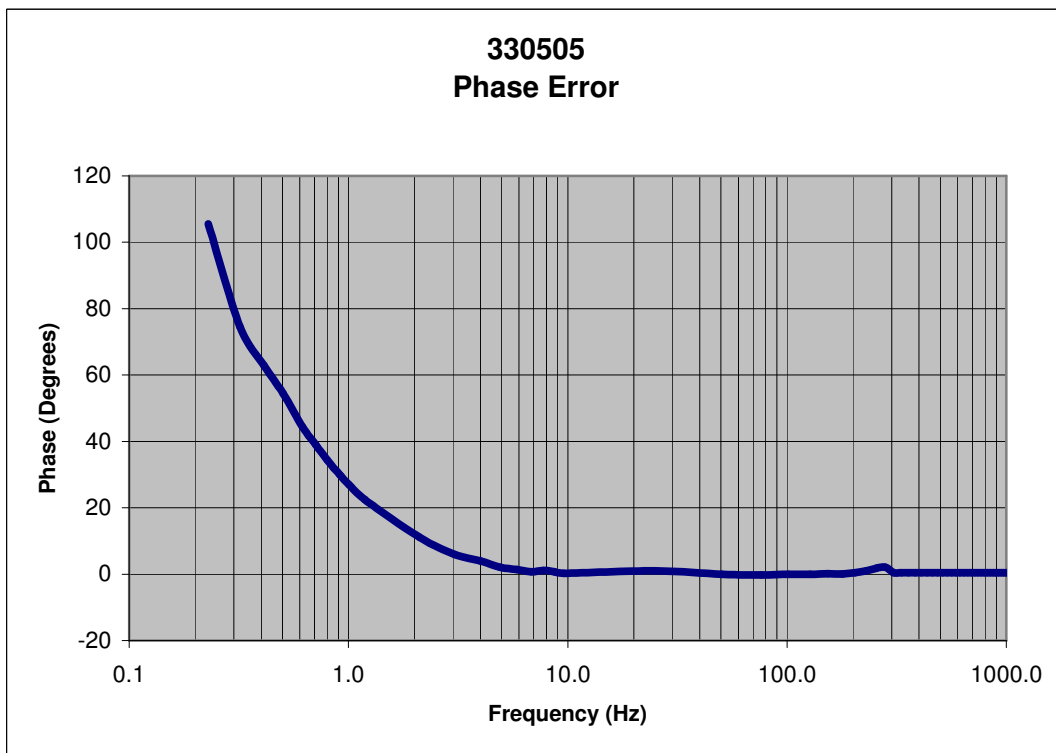
Figure 4: Typical Velocity Phase Error
