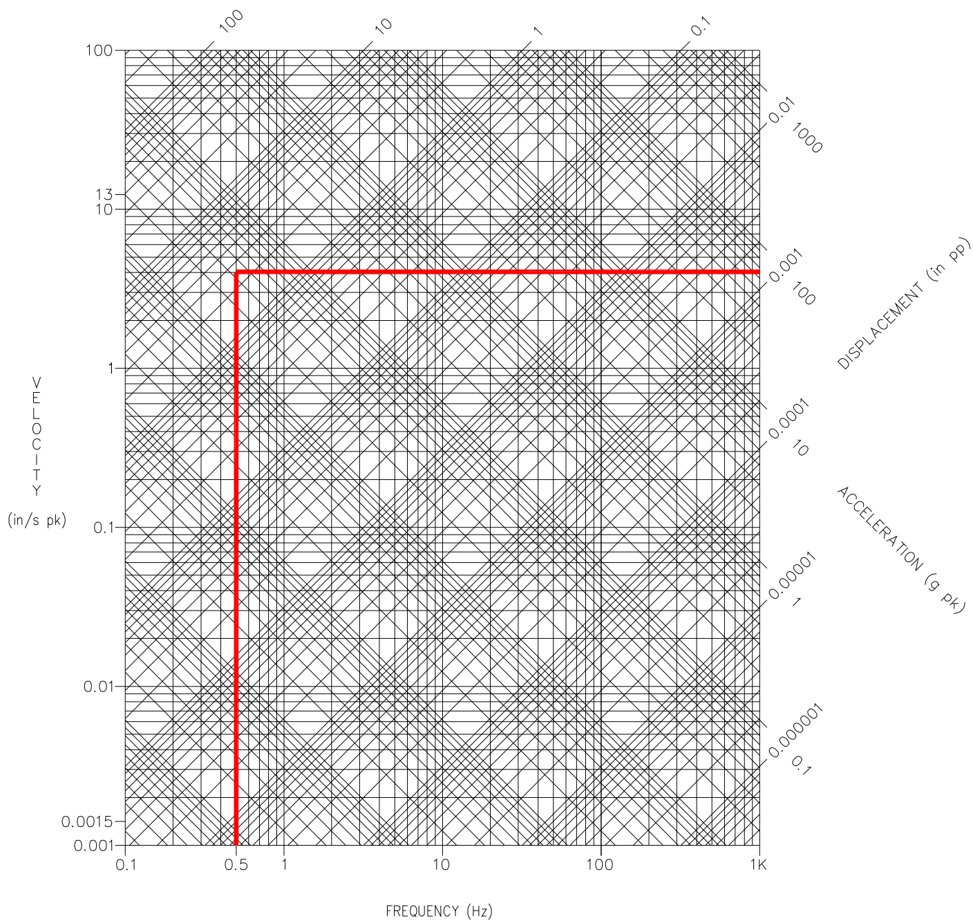
Figure 1: 330505 Vibration Nomograph
